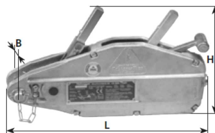
Abmessungen / Dimensions / Dimensions L = 352 mm | B = 101 mm | H = 210 mm
