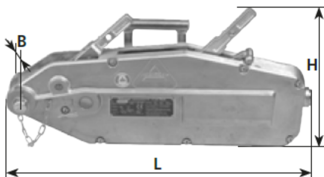
Abmessungen / Dimensions / Dimensions L = 683 mm B = 148 mm H = 330 mm
